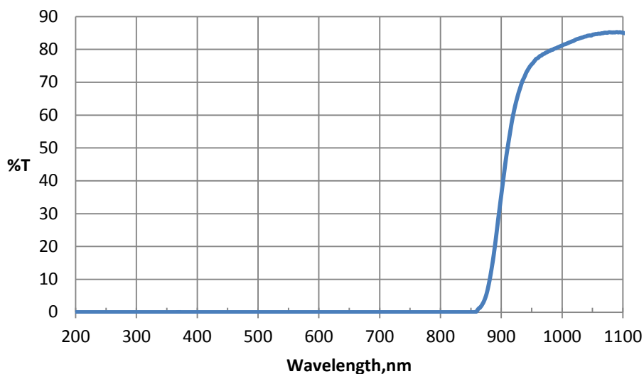
Transmittance spectrum of Luminate 7276F (1.3 mm)
