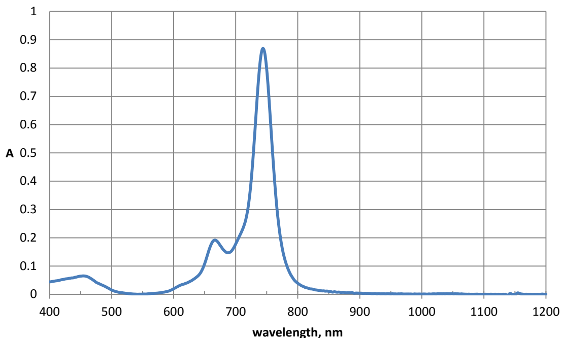
absorbance spectrum of Epolight 6860 in chloroform
