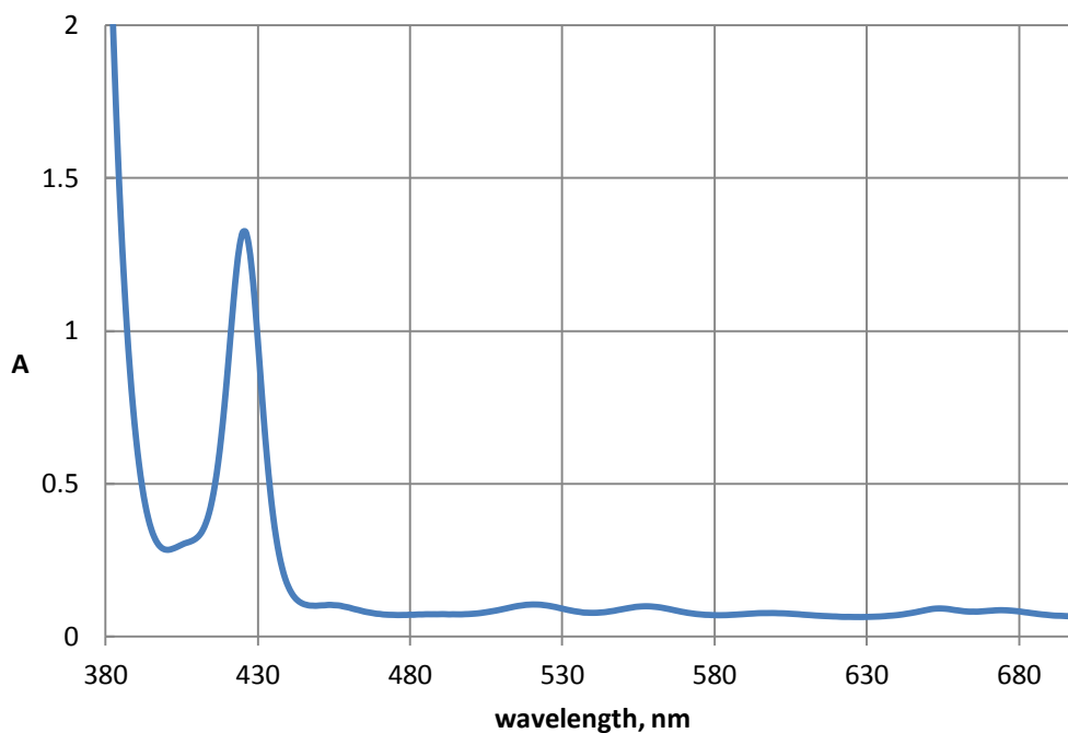
Absorbance spectrum Epolight 5851 in polycarbonate
