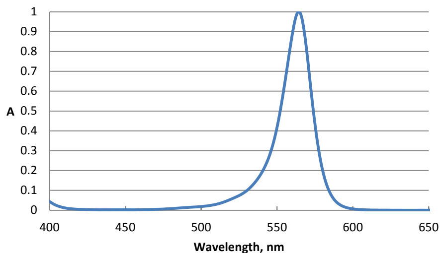
Absorbance spectrum Epolight 5840 in chloroform
